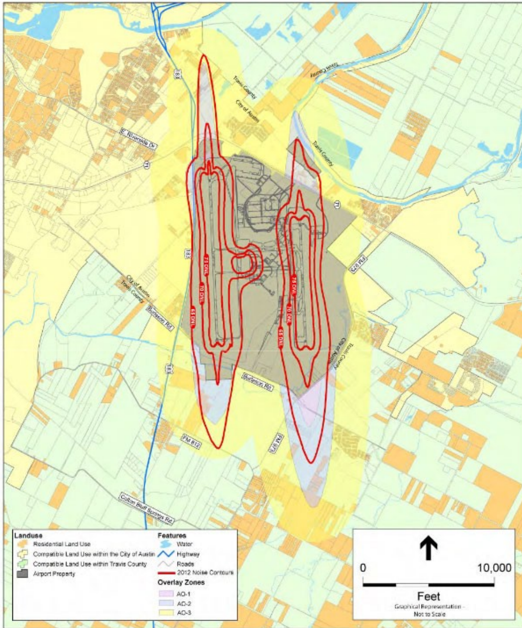
Figure 9.8 Existing Airport Overlay Zones with 2012 Noise Contours
